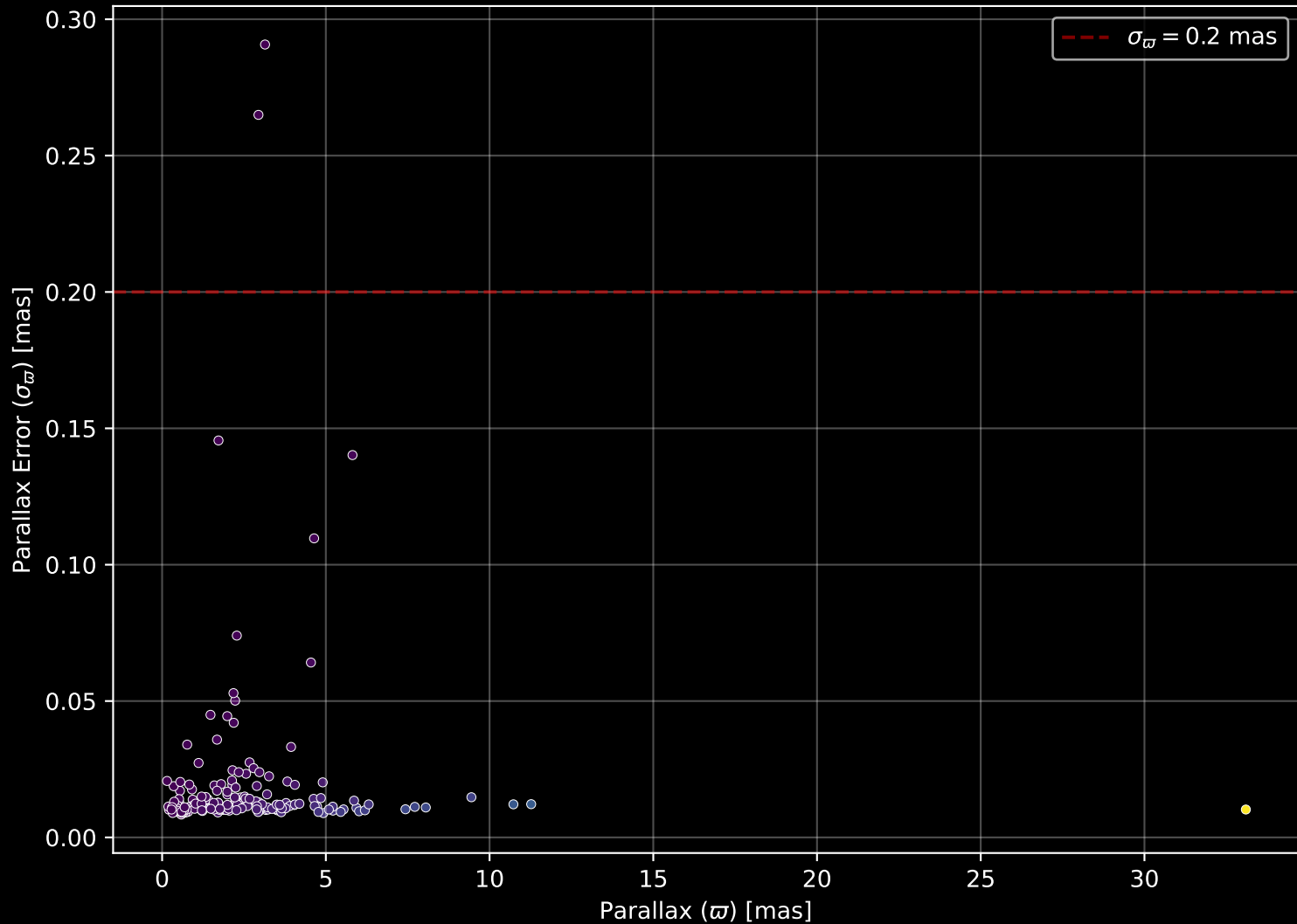
APOGEE DR17 Field: [CVZ_OB17_btx] Parallax Quality (n= 186)
