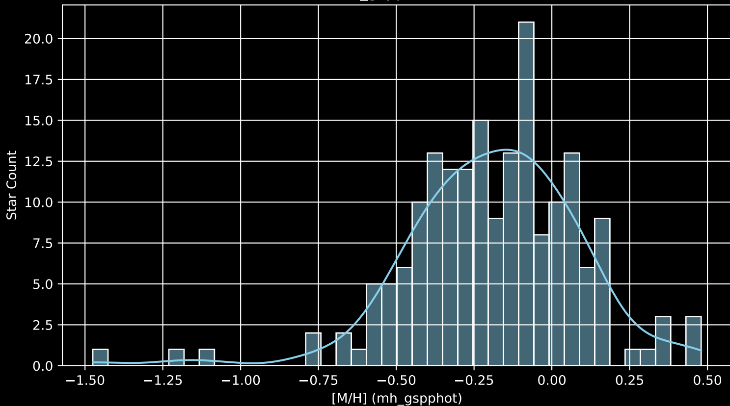
APOGEE DR17 Field: [CVZ_OB17_bt [M/H] (mh_gspphot) (n= 183)
