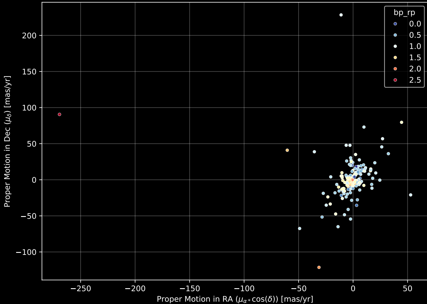
APOGEE DR17 Field: [CVZ_OB17_btx] Proper Motion Diagram (n= 186)
