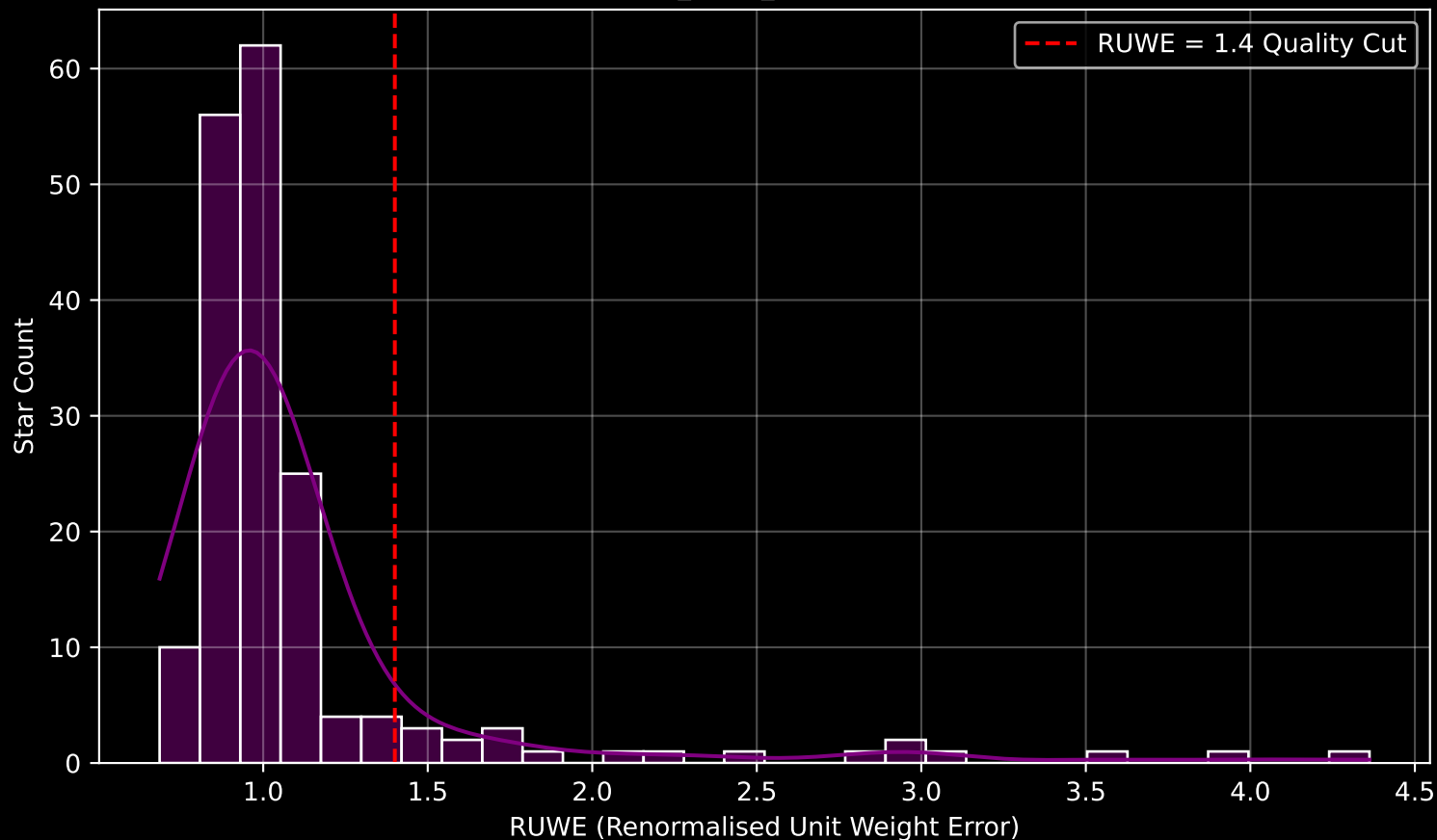
GAPOGEE DR17 Field [CVZ_OB17_btx] RUWE Distribution (n= 180)
