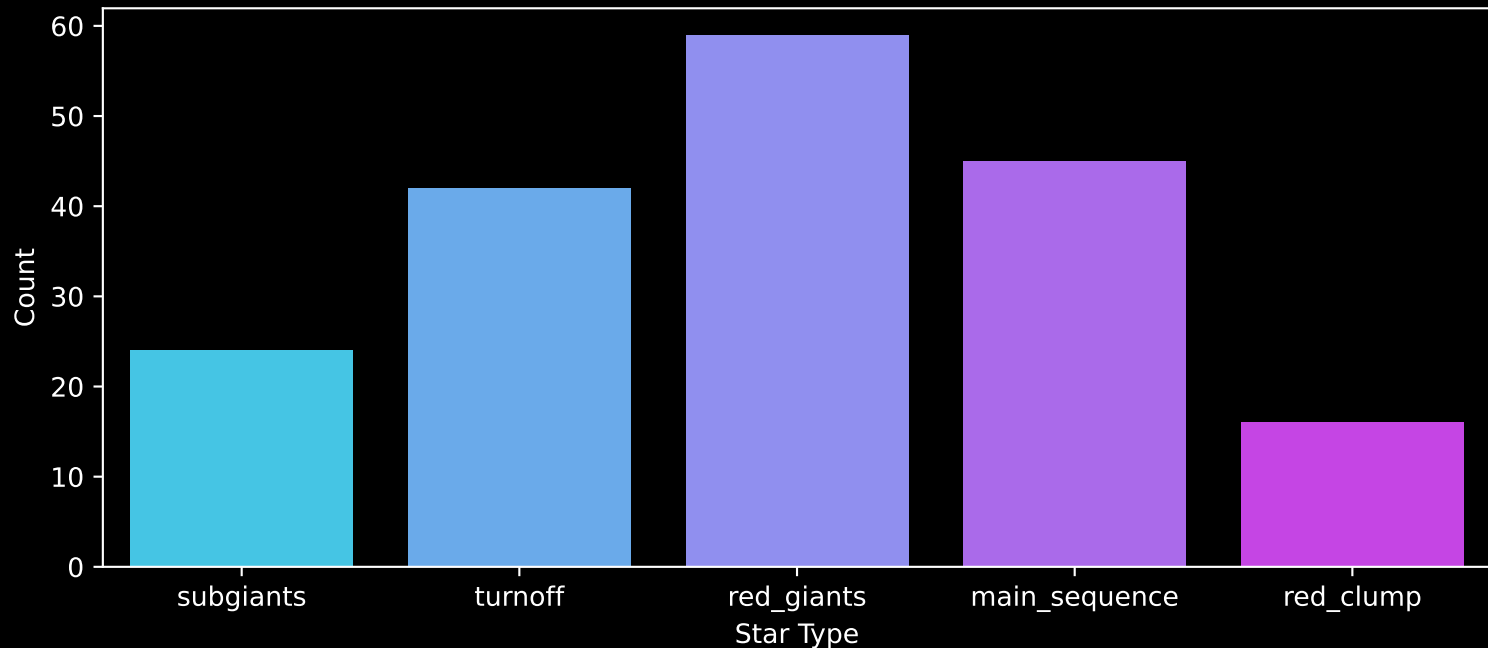
APOGEE DR17 Field: [CVZ_OB17_btx] Count plot of Star Type
